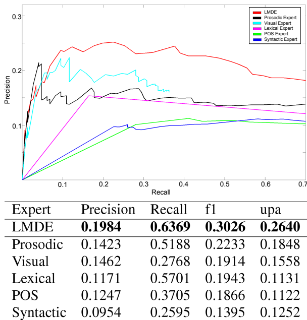
Fig. 7. Comparison of individual experts with our LMDE model. Top: Recall (x-axis) v.s. Precision (y-axis) values for different threshold values. Bottom: Precision, Recall, F1 and UPA scores of corresponding models for selected amount of backchannel.
