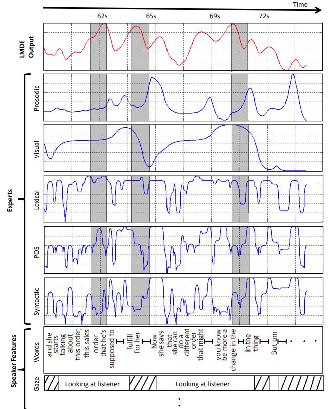
Fig. 9. Output probabilities from LMDE and individual experts for two different sub-sequences. The gray areas in the graph correspond to ground truth backchannel feedbacks of the listener.
