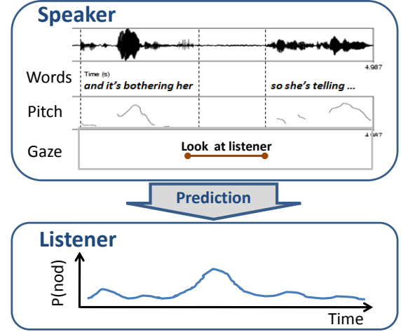
Fig. 2. Example of multimodal prediction model: listener nonverbal backchannel prediction based on speaker's speech and visual gestures. As the speaker says the word her , which is the end of the clause ( her is also the object of the verb bothering ), and lowers the pitch while looking back at the listener and eventually pausing, the listener is then very likely to head nod (i.e., nonverbal backchannel).
